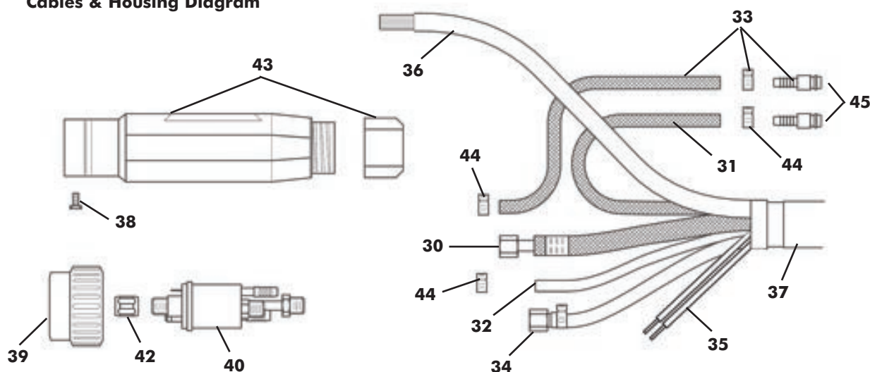
Cables & Housing Diagram
