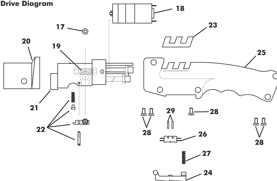
Handle & Drive Diagram
