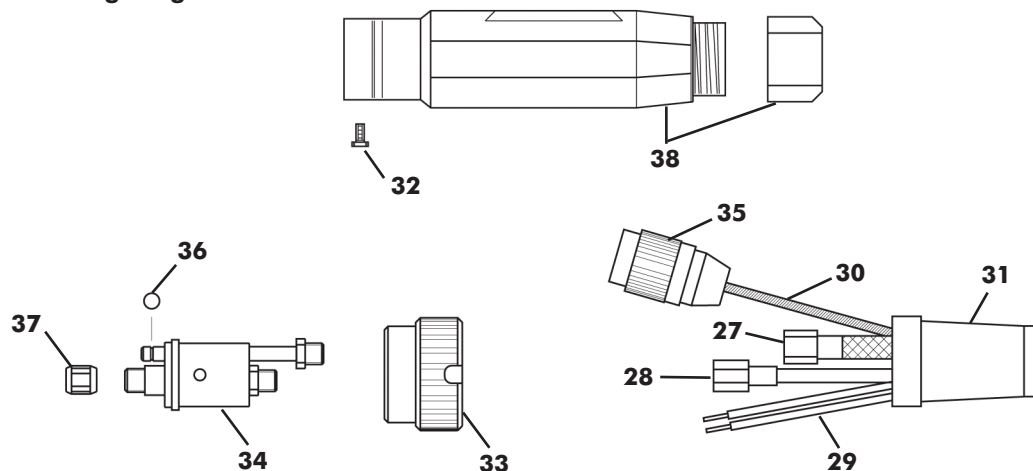
Cables & Housing Diagram
