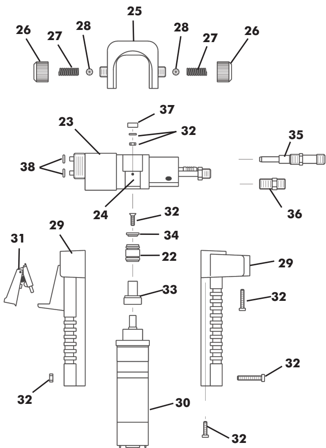
Handle & Drive Diagram
